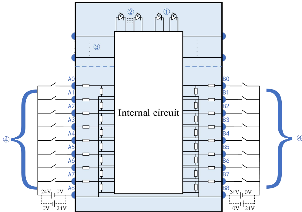
① System Indicator Light ② Channel indicator light light ③ backplane bus ④ Input channel& wiring
