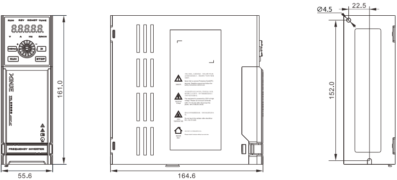
VHL-20P4/20P7/40P4/40P7/41P5-B
