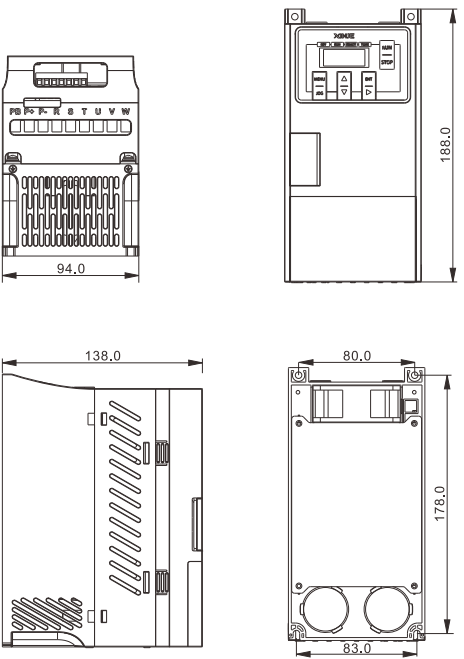
VH5-20P7/21P5/22P2/40P7/41P5/42P2/43P7-B
