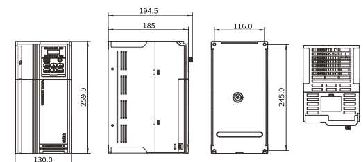
VH1-4011/4015-B
