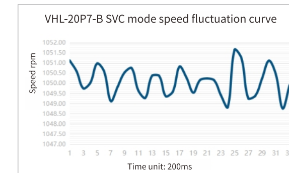
VHL inverter speed fluctuation \pm 0.3\%
