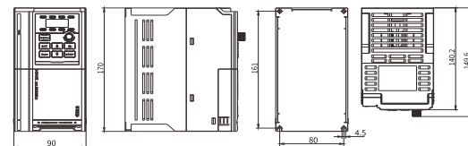
VH1-4011/4015-B
