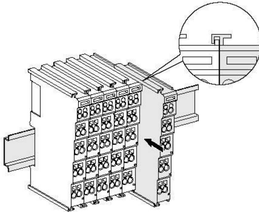
Figure 2.2 GCAN-PLC-511 installation
