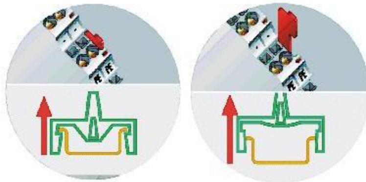
Figure 2.3 GCAN-PLC-511 self-locking mechanism
